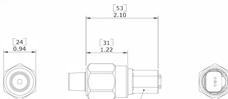
DT04-2P, 2 POLE RECEPTACLE MATING; DT06-2S, 2 POLE PLUG
